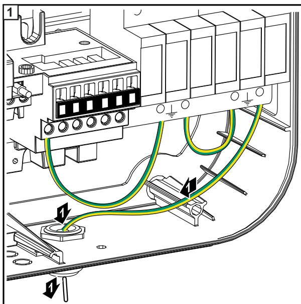
M16 cable gland - enclosed
