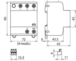
Dimension drawing DSH B TNC 255 FM
