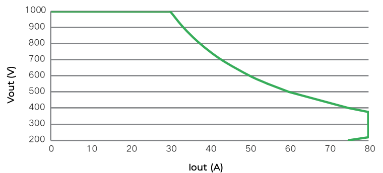
VOUT-IOUT CURVE
